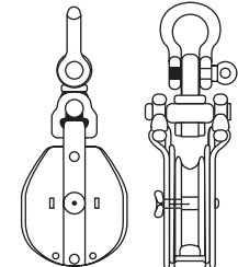
Steel Shell Block with Drilled Swivel Eye & Shackle
