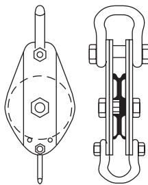
SINGLE SHEAVE BLOCK WITH SHACKLE
