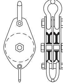
DOUBLE SHEAVE BLOCK WITH SHACKLE
