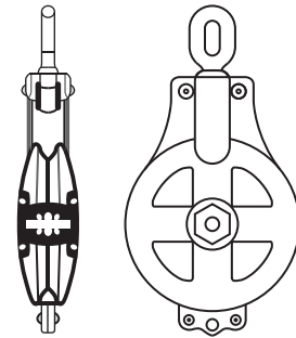
CARGO BLOCK WITH OBLONG EYE
